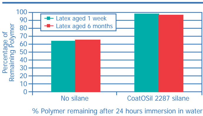
Figure 5: Water Resistance of Acrylic Latex Coating Cured with CoatOSil 2287 Silane
