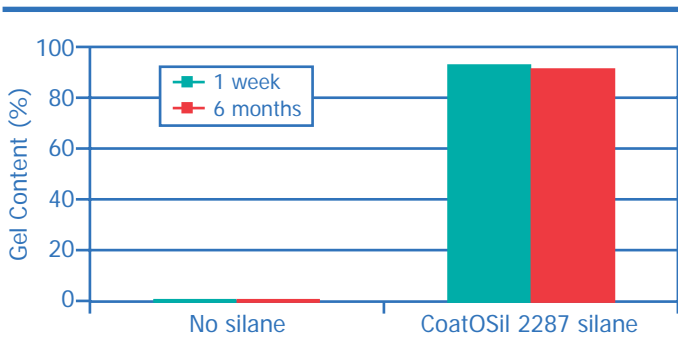
Figure 3: Gel Content of Acrylic Latex Coating Cured with CoatOSil 2287 Silane
