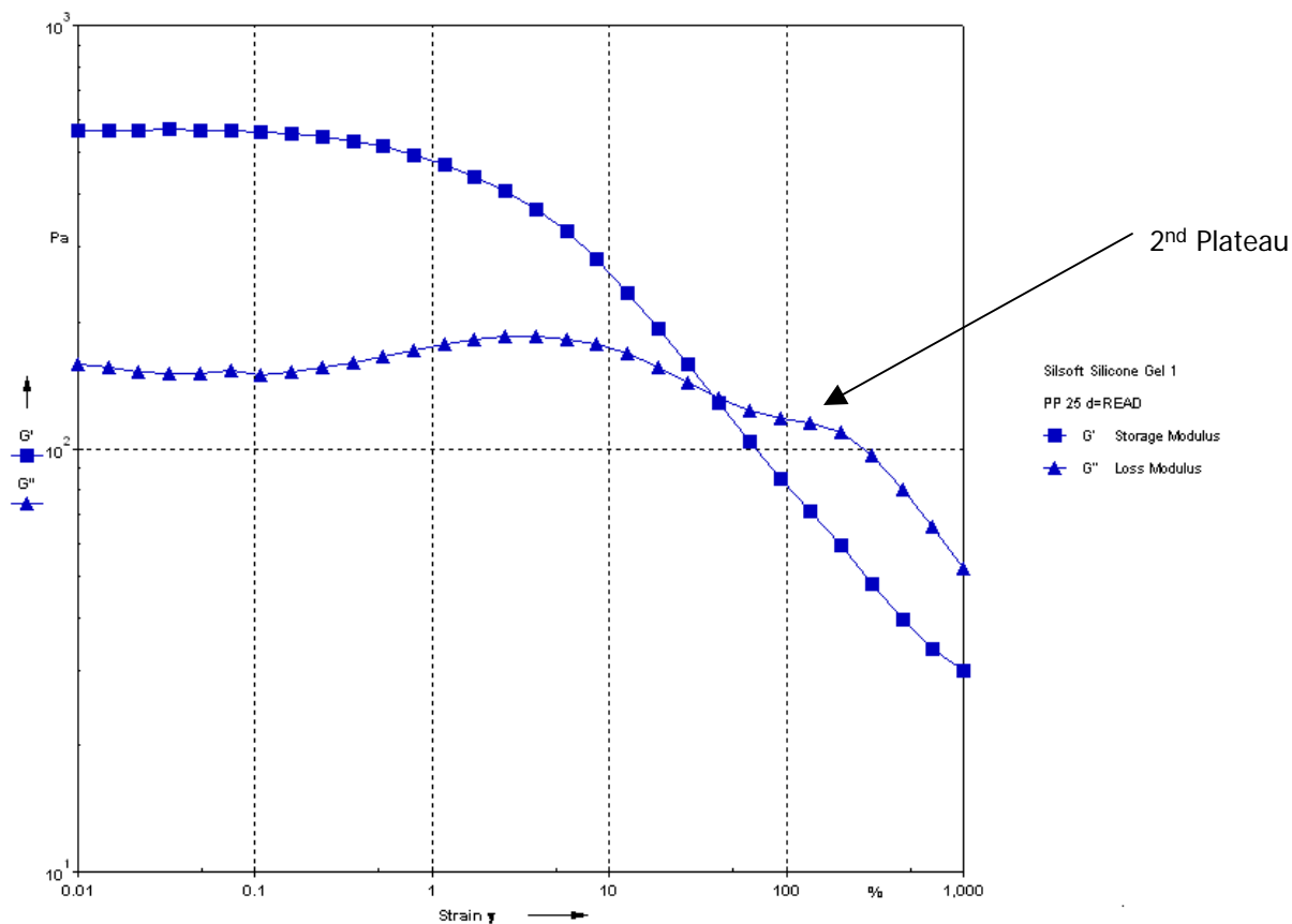
Amplitude Sweep
